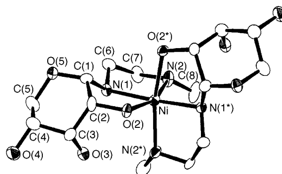
Fig. 10 An ORTEP diagram of the complex cation of [Ni(D-Rib-men) 2 ]Br 2 ·2CH 3 OH·5·2CH 3 OH
